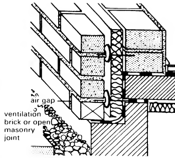
2 Detail at base
